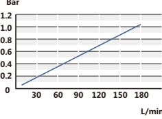
Curve of pressure loss 压力损失曲线
