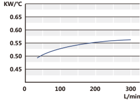
Curve of heat abstraction quantity 散热量曲线
