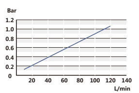
Curve of pressure loss 压力损失曲线
