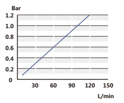
Curve of pressure loss 压力损失曲线
