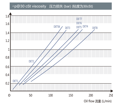
Pressure loss 压力损失 DET1~DET8
