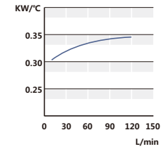
Curve of heat abstraction quantity 散热量曲线
