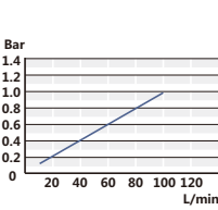
Curve of pressure loss 压力损失曲线
