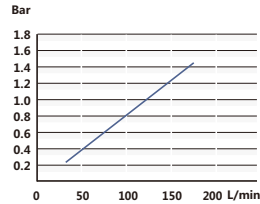
Curve of pressure loss 压力损失曲线
