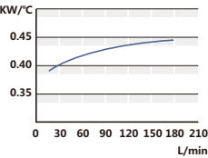
Curve of heat abstraction quantity 散热量曲线
