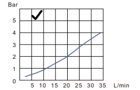
Curve of pressure loss 压力损失曲线
