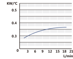
Curve of heat abstraction quantity 散热量曲线
