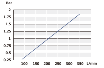
Curve of pressure loss 压力损失曲线
