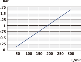
Curve of pressure loss 压力损失曲线
