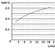
Curve of heat abstraction quantity 散热量曲线
