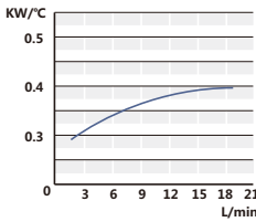
Curve of heat abstraction quantity 散热量曲线
